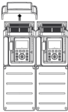
Mounting Type C: Individual IP20
