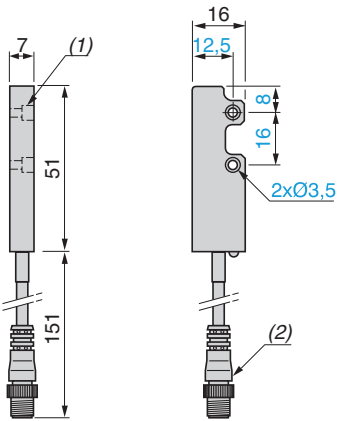
(1) Counterbored: Ø 6 x 3.5 mm. (2) M8 4-pin connector.
