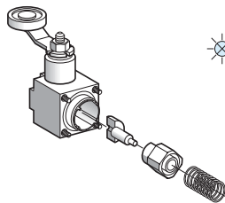
Head ZCK D05
