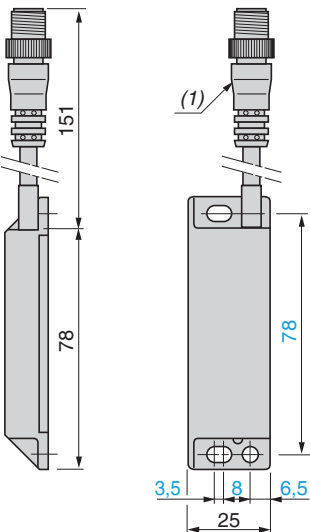
(1) 4 or 6-pin M12 connector.
