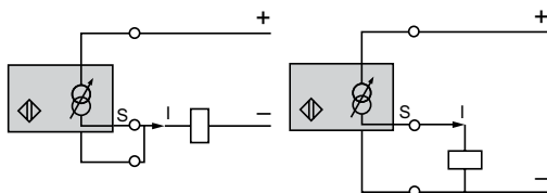
2-wire connection
